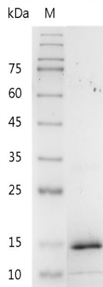
SDS-PAGE analysis of recombinant human BMP-12
